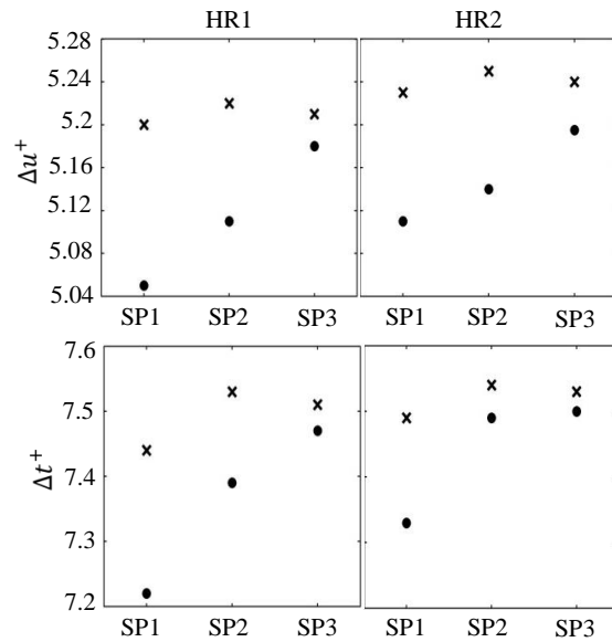
Figure 8. Characteristics of the averaged sweep events in the vicinity of the resonators in the spanwise direction at y^+ = 35 when Re_\theta = 1800 ; (a) sweep intensity and (b) sweep duration with resonator (circle), no-resonator case (cross).
