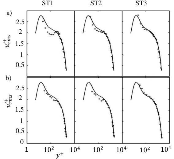
Figure 4. Turbulence intensity profiles within the boundary layer downstream of the resonators at different streamwise locations when Re_\theta=3000 ; a) HR1 and b) HR2; with resonator (circle), no-resonator case (solid line).
