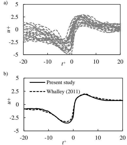
Figure 6. VITA events at y^+ = 35 for unexcited boundary layer when Re_\theta = 1800 ; (a) sweep events and (b) averaged VITA sweep event.
