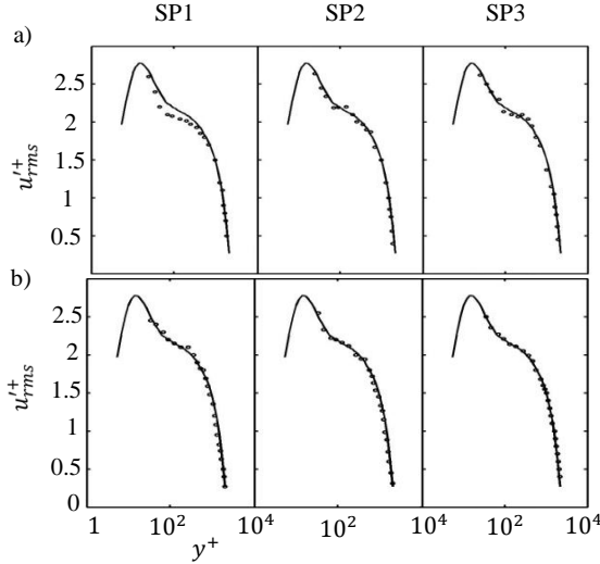
Figure 5. Turbulence intensity profiles within the boundary layer downstream of the resonators at different spanwise locations when Re_\theta = 1800 ; a) HR1 and b) HR2; with resonator (circle), no-resonator case (solid line).
