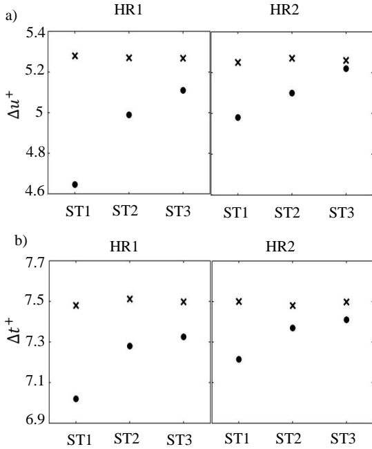
Figure 7. Characteristics of the averaged sweep events downstream of the resonators in the streamwise direction at y^+ = 35 when Re_\theta = 1800 ; (a) sweep intensity and (b) sweep duration with resonator (circle), no-resonator case (cross).
