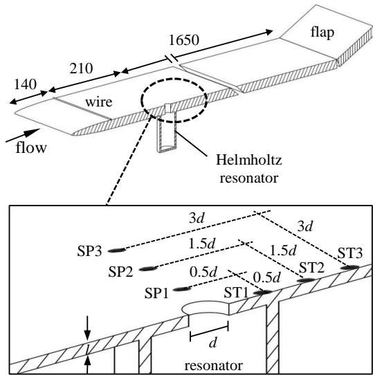
Figure 1. Schematic of cross-section experimental setup and the locations for measurements.
