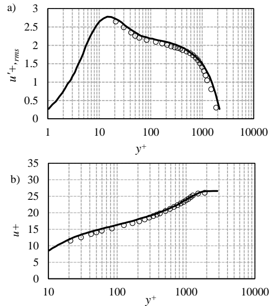
Figure 2. Streamwise velocity profiles of the incoming turbulent boundary layer upstream of the resonator at Re_\theta = 5000 , a) velocity fluctuating; b) mean velocity; (solid line) DNS by Sillero et al. (2013) and (circle) present investigation.
