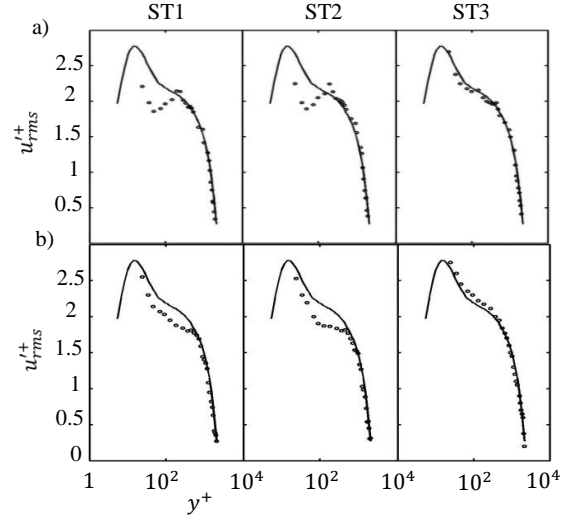
Figure 3. Turbulence intensity profiles within the boundary layer downstream of the resonators at different streamwise locations when Re_\theta=1800 ; a) HR1 and b) HR2; with resonator (circle), no-resonator case (solid line).
