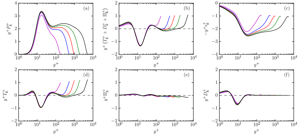
Figure 1. Production, transport and dissipation of turbulent kinetic energy: (a) Production (b) Transport (Turbulent+Pressure+Viscous) (c) Dissipation (d) Turbulent transport (e) Pressure transport (f) Viscous transport. R180: — (Magenta), R550: — (Blue), R1000: — (Red), R2000: — (Green), R5200: — (Black)
