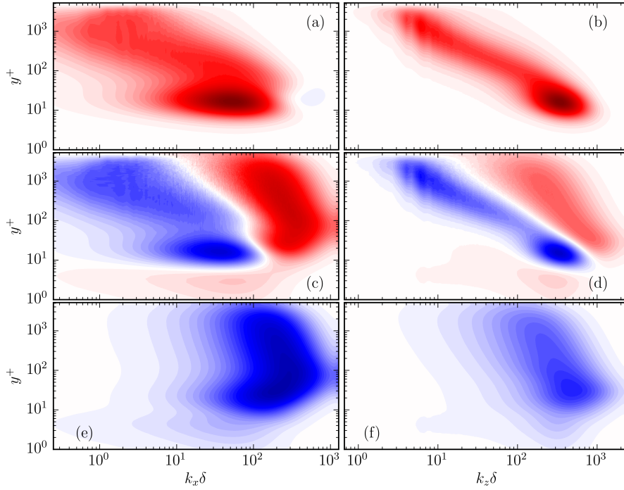
Figure 2. One-dimensional spectral density of production, transport and dissipation of turbulent kinetic energy for case R5200: (a) y^+ k_x E_{x,P_k} (b) y^+ k_z E_{z,P_k} (c) y^+ k_x (E_{x,T_k} + E_{x,D_k} + E_{x,\Pi_k}) (d) y^+ k_z (E_{z,T_k} + E_{z,D_k} + E_{z,\Pi_k}) (e) -y^+ k_x E_{x,\epsilon_k} (f) -y^+ k_z E_{z,\epsilon_k} . Red is positive, white is zero and blue is negative.
