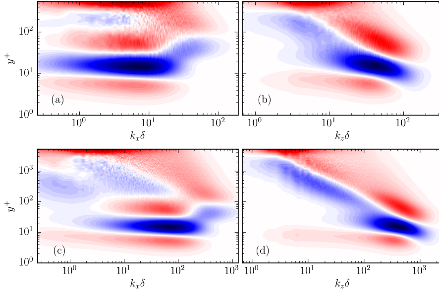
Figure 4. One-dimensional spectral density of transport of turbulent kinetic energy, T_{k,1} (see eq (2)), for case R550(Top) and R5200(Bottom): (a) y^+ k_x E_x, T_{k,1} (R550) (b) y^+ k_z E_z, T_{k,1} (R550) (c) y^+ k_x E_x, T_{k,1} (R5200) (d) y^+ k_z E_z, T_{k,1} (R5200). Red is positive, white is zero and blue is negative.
