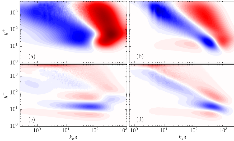
Figure 3. One-dimensional spectral density of turbulent transport of turbulent kinetic energy for case R5200: (a) y^+ k_x E_x, T_{k,0} (b) y^+ k_z E_z, T_{k,0} (c) y^+ k_x E_x, T_{k,1} (d) y^+ k_z E_z, T_{k,1} . Red is positive, white is zero and blue is negative.
