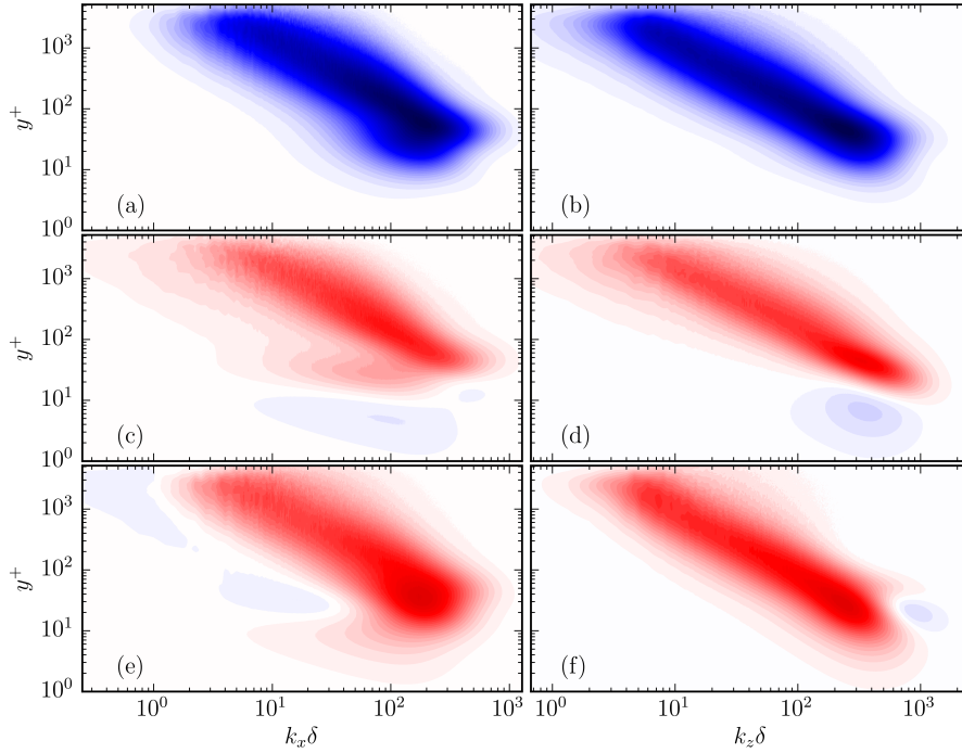
Figure 5. One-dimensional spectral density of pressure strain of velocity fluctuations: (a) y^+ k_x E_{x, \Pi_{s,uu}} (b) y^+ k_z E_{z, \Pi_{s,uu}} (c) y^+ k_x E_{x, \Pi_{s,vv}} (d) y^+ k_z E_{z, \Pi_{s,vv}} (e) y^+ k_x E_{x, \Pi_{s,ww}} (f) y^+ k_z E_{z, \Pi_{s,ww}} , R5200 Red is positive, white is zero and blue is negative.
