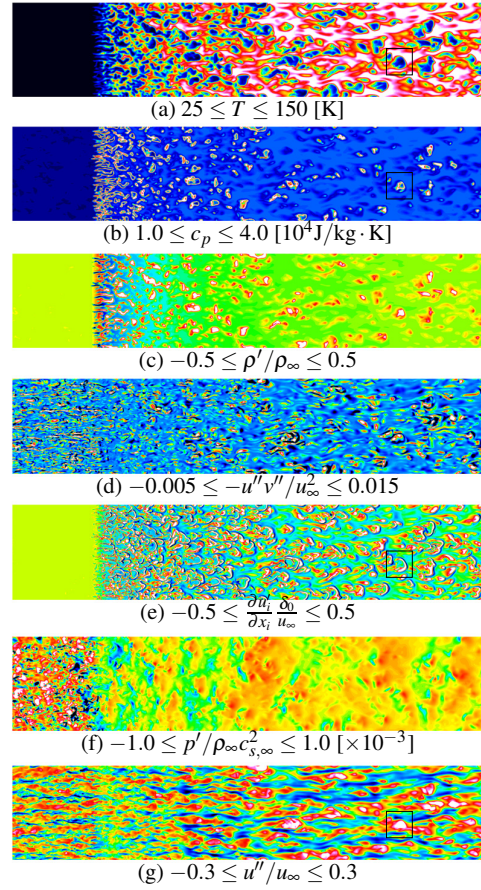
Figure 7. Instantaneous snapshots of the transcritical heated boundary layer in wall-parallel planes at y/\delta \approx 0.05 in the region of 0 \leq x/\delta_0 \leq 30 and 0 \leq z/\delta_0 \leq 6 (whole right-side domain in Fig. 4) under p = 2 MPa and T_w = 200K conditions.
