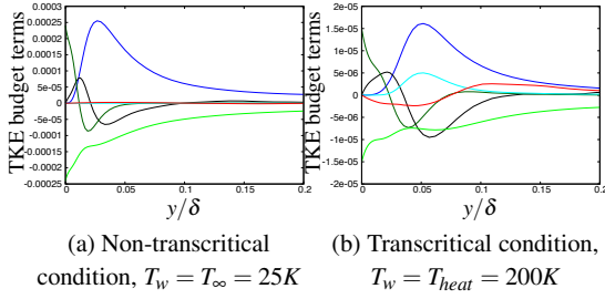
Figure 6. Turbulent kinetic energy budget in unheated non-transcritical and heated transcritical turbulent boundary layers at supercritical pressure of p = 2 MPa. Blue, production P ; black, turbulent transport T ; dark green, viscous diffusion D_v ; light green, energy dissipation D_d ; cyan, mass flux contribution M ; red, pressure dilatation \Pi_d .
