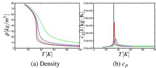
Figure 2. Variable thermodynamic properties for parahydrogen using REFPROP (NIST Standard Reference Database 23, Version 9.0). Density and specific heat in terms of the temperature at constant pressure. Black, p = 1.2858\text{MPa} ; red, p = 1.5\text{MPa} ; blue, p = 2.0\text{MPa} ; green, p = 4.0\text{MPa} .
