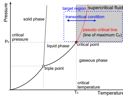
Figure 1. Transcritical condition through the pseudo-critical temperature in a phase diagram.
