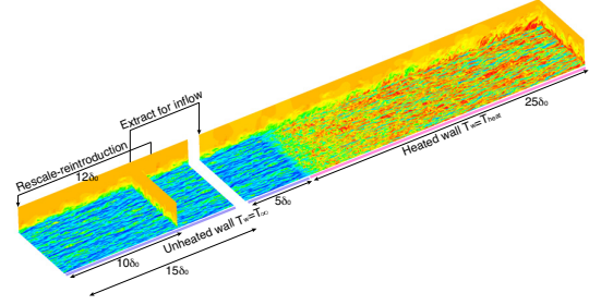
Figure 4. Direct numerical simulation of transcritical heated parahydrogen turbulent boundary layer on a zero-pressure-gradient flat plate under supercritical pressure conditions. Mach number contours, and wall-parallel (at y^+ \approx 20 ) planes.
