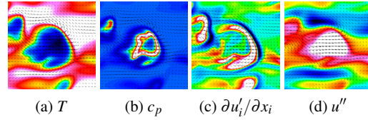
Figure 8. Zoomed instantaneous snapshots overlaid with velocity fluctuation vectors (every third grid point) in the region of the black solid-line boxes in Fig. 7.
