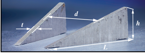
Figure 1. (Photo published in Shahinfar et al. , 2012) A photo of a MVG pair with triangular blades. The geometrical parameters: h = 1.1 , d = L = 3.25 and t = 0.3 (mm).
