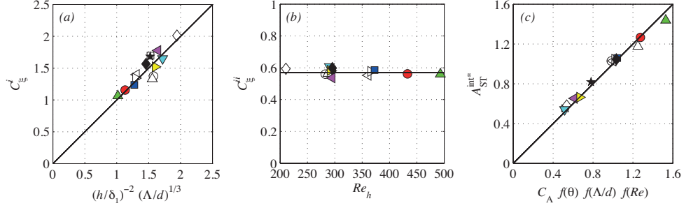
Figure 4. (Figure published in Sattarzadeh & Fransson, 2015). The coefficients C_\xi^i , C_\xi^{ii} and A_{ST}^{int*} , as defined by Eqs. 1 – 4, in (a), (b) and (c), respectively, versus the proposed scaling. The coefficients are determined by means of least square fit of the data to Eq. 1. f(\theta) , f(\Lambda/d) and f(Re) in (c) are described in the running text.
