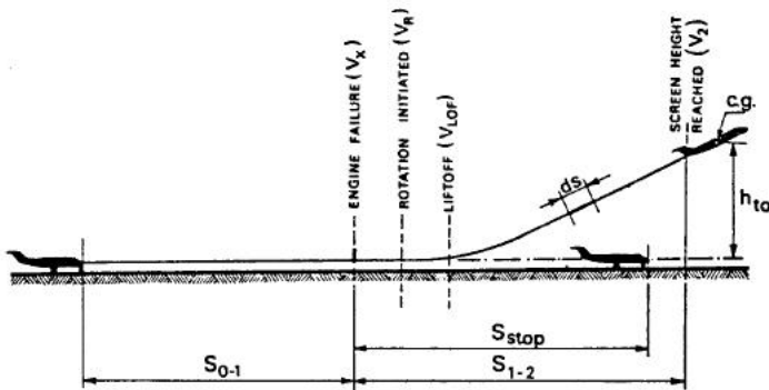
Fig. 5-16. Phases during the takeoff with engine failure
