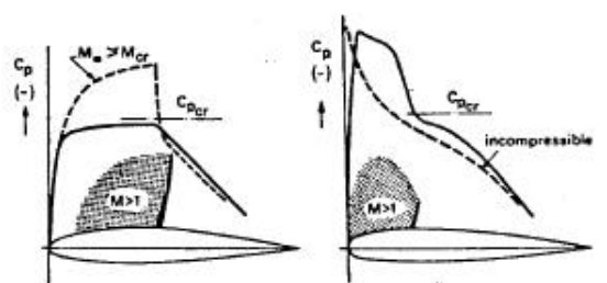
a. Conventional section with roof-top pressure distribution
