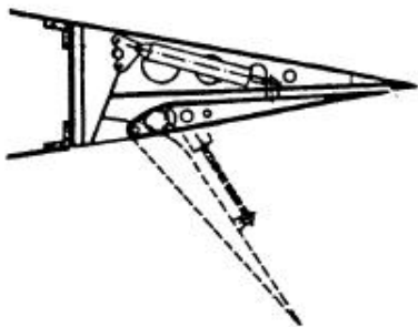
Fig. 25a. Split flap
