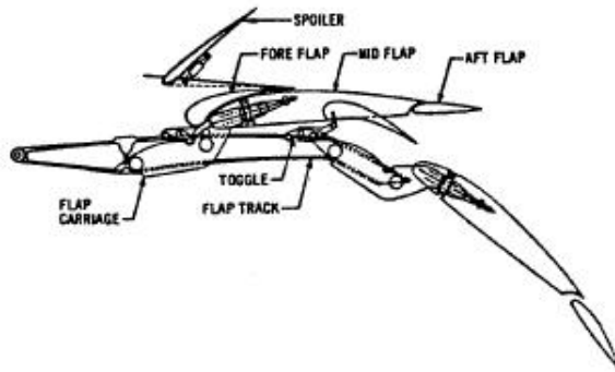
Fig. 7-25h. Triple slotted flap (Boeing 727)
