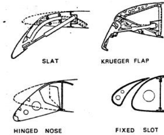
Fig. 7-26. Leading-edge high-lift devices.
