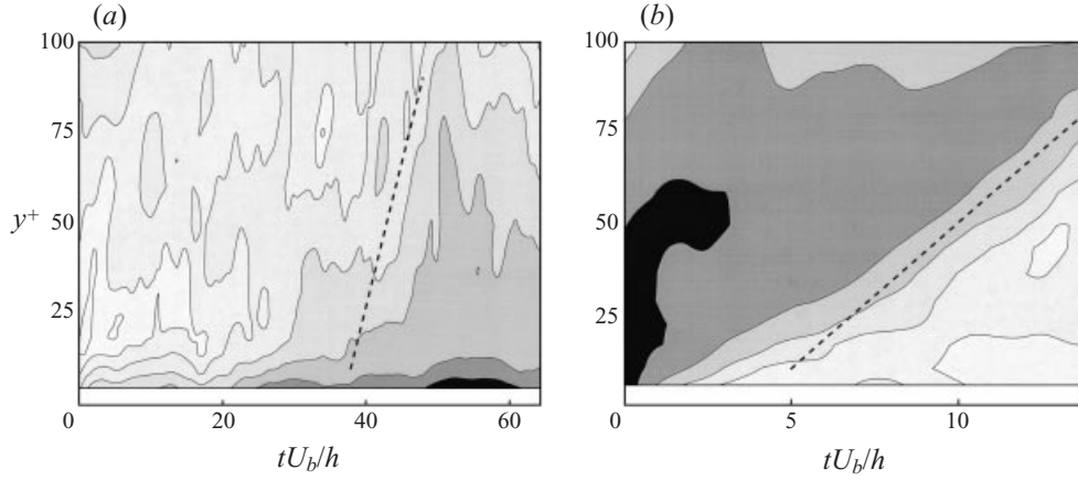
FIGURE 14. Evolution of wall-normal distribution of the spanwise correlation length L_{uu,z}^+ . Contours are L_{uu,z}^+ = 0.5(\times 2)32 , going from light to dark. (a) Start-up case P3. (b) Shutdown case I2. The dotted lines in both plots have slope dy^+/dt^+ \approx 0.6 .
