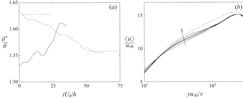
FIGURE 13. (a) Variation of the form factor of the boundary layer over the porous wall during the transition: —, shutdown case I2; — — —, start-up case P3; — · —, mean form factor for case I1; · · · · ·, mean form factor for case P2. (b) Time variation of the instantaneous mean velocity profile for case I2, normalized in the wall units of the porous wall at the beginning of the shut-down. Times are U_b t/h = 0, 3.5, 6.4, 10, 13.3 , increasing in the direction of the arrow. — — —, Asymptotic profile of case I1, in the same normalization.
