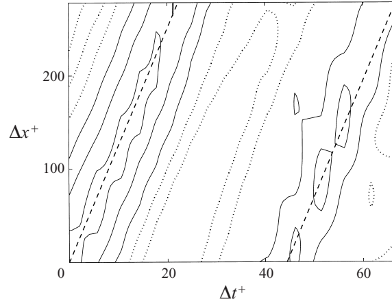
FIGURE 8. Space-time correlation function of the spanwise-averaged fluctuations \bar{u} , for the porous case P1. Contours are R_{ii} = -0.7(0.1)0.8 , and the dotted contours are negative. The dashed line corresponds to an advection velocity U_c^+ = 12.5 , based on the friction velocity of the bottom wall.
