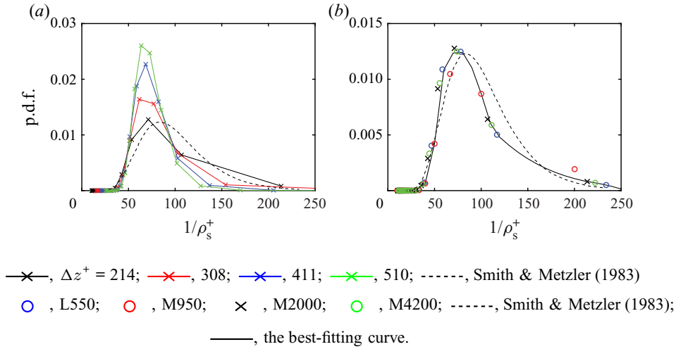
Figure 7. (a) Probability density function of the streak density at different \Delta z^+ in case M2000: black, \Delta z^+ = 214 ; red, \Delta z^+ = 308 ; blue, \Delta z^+ = 411 ; green, \Delta z^+ = 510 ; dashed, Smith & Metzler (1983). (b) Probability density function of the streak density distributions at different Re_\tau and \Delta z^+ \approx 200 : blue circles, L550; red circles, M950; black crosses, M2000; green circles, M4200; dashed line, Smith & Metzler (1983); full line, the best-fitting curve.
