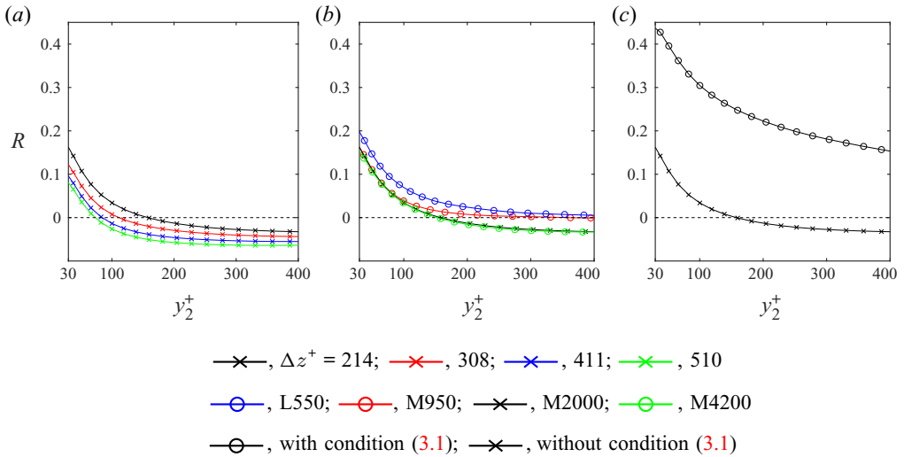
Figure 8. (a) Correlation R(\rho_s, \tilde{v}) at different \Delta z^+ in case M2000: black, \Delta z^+ = 214 ; red, \Delta z^+ = 308 ; blue, \Delta z^+ = 411 ; green, \Delta z^+ = 510 . (b) As in (a) for different Re_\tau and \Delta z^+ \approx 200 : blue, L550; red, M950; black, M2000; green, M4200. (c) Correlation for \Delta z^+ = 214 in case M2000: circles, with condition (3.1); crosses, without condition (3.1).
