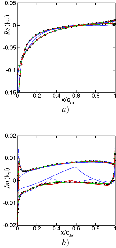
Figure 13. SKIN FRICTION COEFFICIENT OF 30 % BLADE SECTION COMPUTED WITH TD AND FIVE HB ANALYSES (LINE LEGEND AS IN FIG. 12-a): a) REAL PART, b) IMAGINARY PART.
