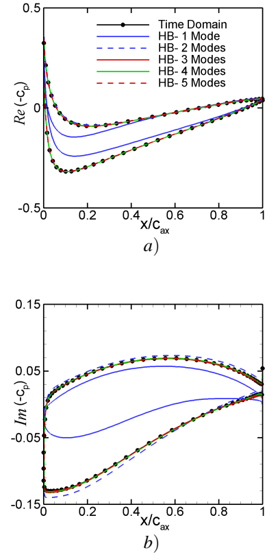
Figure 12. PRESSURE COEFFICIENT OF 30 % BLADE SECTION COMPUTED WITH TD AND FIVE HB ANALYSES: a) REAL PART, b) IMAGINARY PART.
