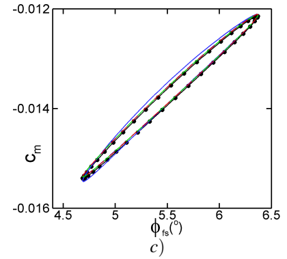
Figure 6. HYSTERIS FORCE LOOPS OF 90 % BLADE SECTION COMPUTED WITH TD AND FIVE HB ANALYSES (LINE LEGEND AS IN FIG. 10): a) LIFT COEFFICIENT, b) DRAG COEFFICIENT, c) PITCHING MOMENT COEFFICIENT.
