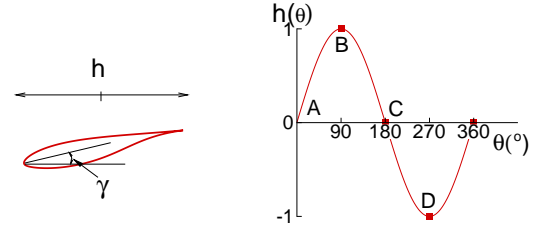
Figure 3. HARMONIC MOTION OF HAWT BLADE SECTION CORRESPONDING TO YAWED INFLOW.
