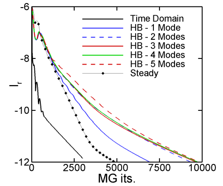
Figure 14. CONVERGENCE HISTORIES OF TD, HB AND STEADY ANALYSES FOR 30 % BLADE SECTION
