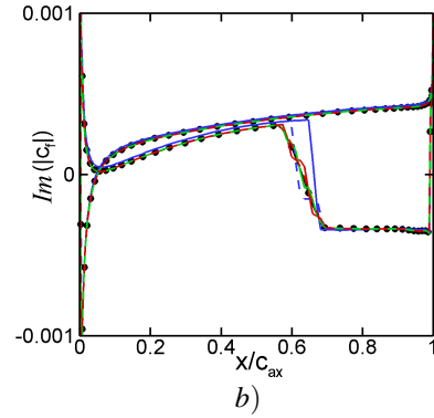
Figure 8. SKIN FRICTION COEFFICIENT OF 90 % BLADE SECTION COMPUTED WITH TD AND FIVE HB ANALYSES (LINE LEGEND AS IN FIG. 12-a): a) REAL PART, b) IMAGINARY PART.
