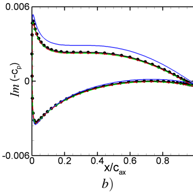
Figure 7. PRESSURE COEFFICIENT OF 90 % BLADE SECTION COMPUTED WITH TD AND FIVE HB ANALYSES: a) REAL PART, b) IMAGINARY PART.
