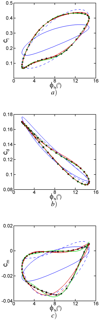
Figure 11. HYSTERIS FORCE LOOPS OF 30 % BLADE SECTION COMPUTED WITH TD AND FIVE HB ANALYSES (LINE LEGEND AS IN FIG. 10): a) LIFT COEFFICIENT, b) DRAG COEFFICIENT, c) PITCHING MOMENT COEFFICIENT.
