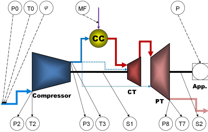
FIGURE 2. GAS PATH INPUT AND OUTPUT SIGNALS.
